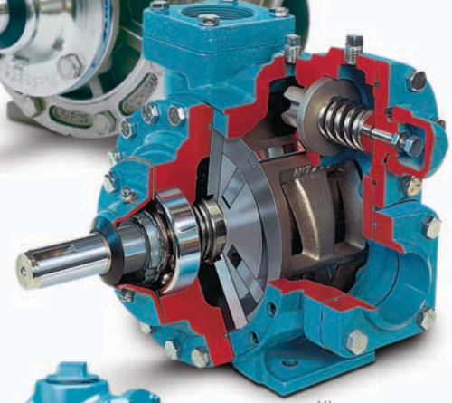
XL Sliding Vane Pump
